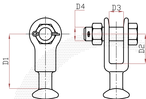
Ball Clevis
