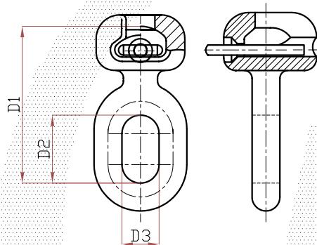
Socket Eye
