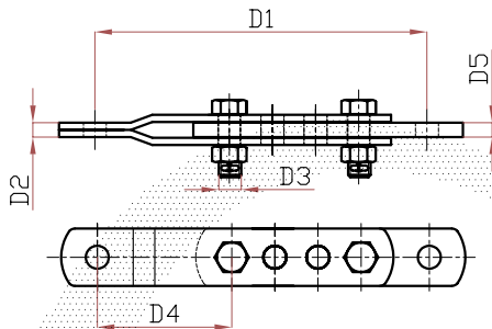
Tongue-Tongue
