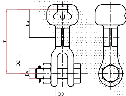
Socket Clevis
