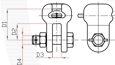
Socket Clevis
