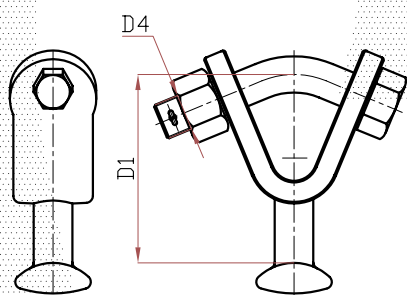
Y_Ball Clevis
