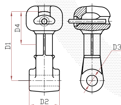
Socket Eye
