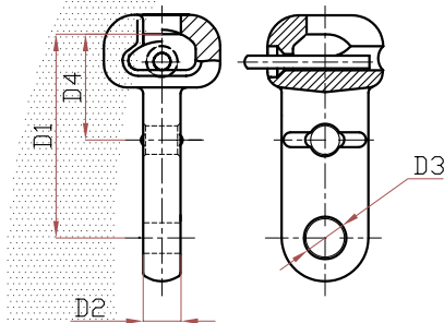
Socket Eye
