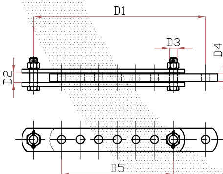
Clevis-Tongue
