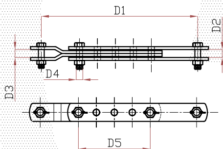
Clevis-Clevis
