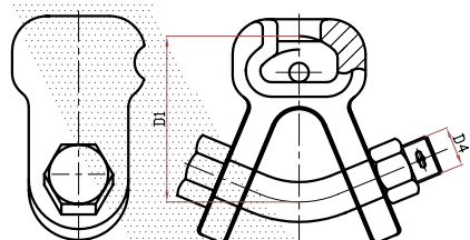
Y_Socket Clevis
