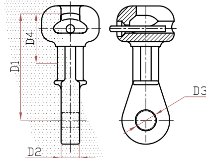
Socket Eye
