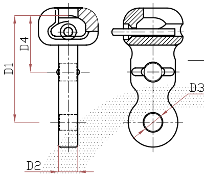
Socket Eye
