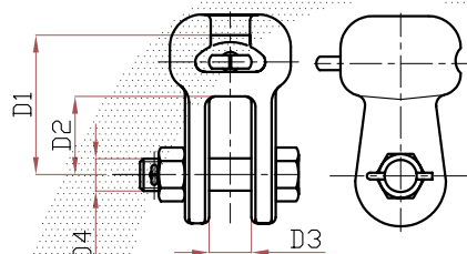
Socket Clevis
