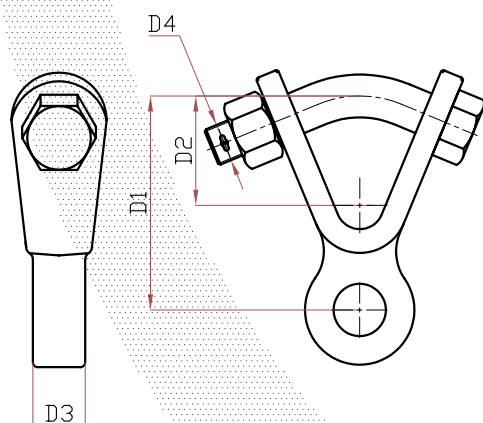
Y-Clevis Eye
