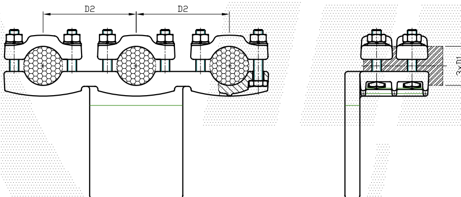
Pad to three wires
