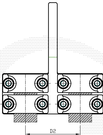
Flat to two wires
