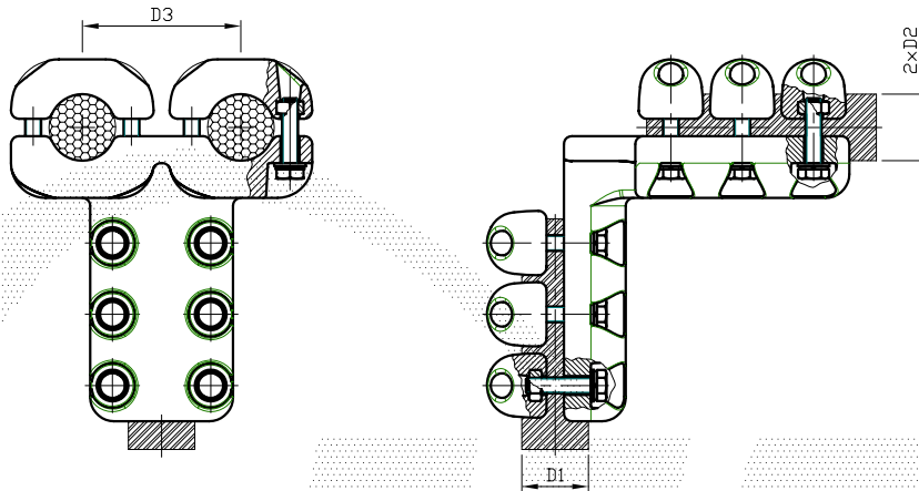
(Wire/Stud) to two wires
