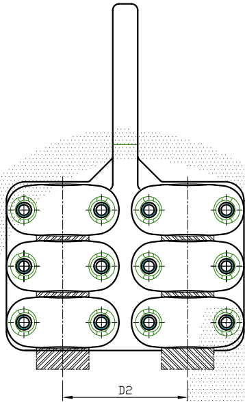
Flat to two wires
