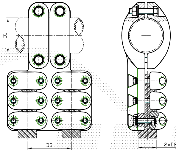
Tube to two wires
