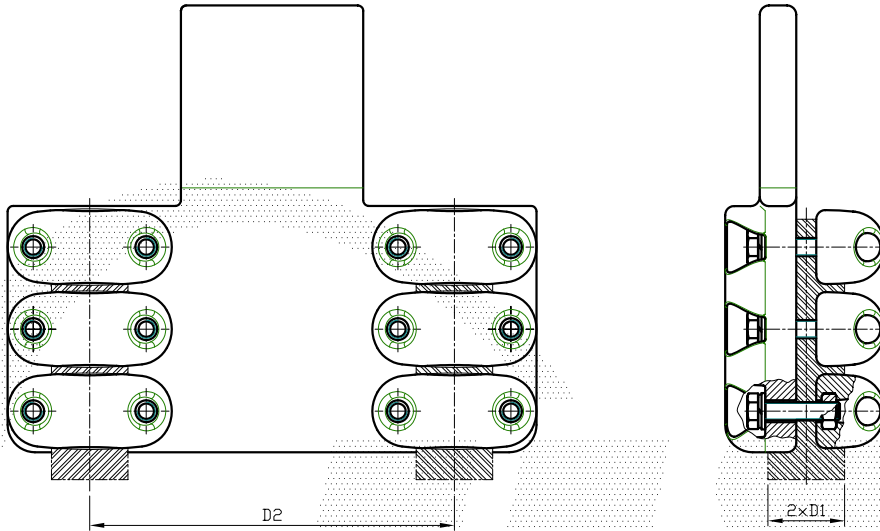
Flat to two wires
