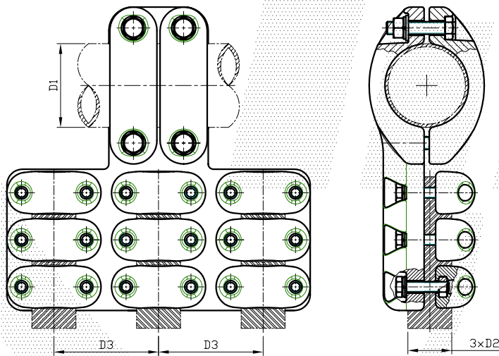
Tube to three wires
