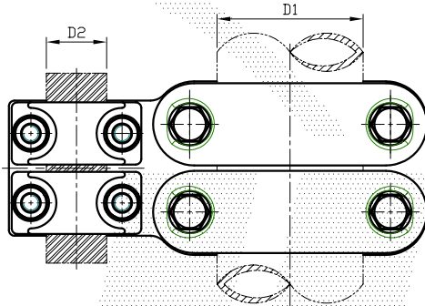
Tube to wire
